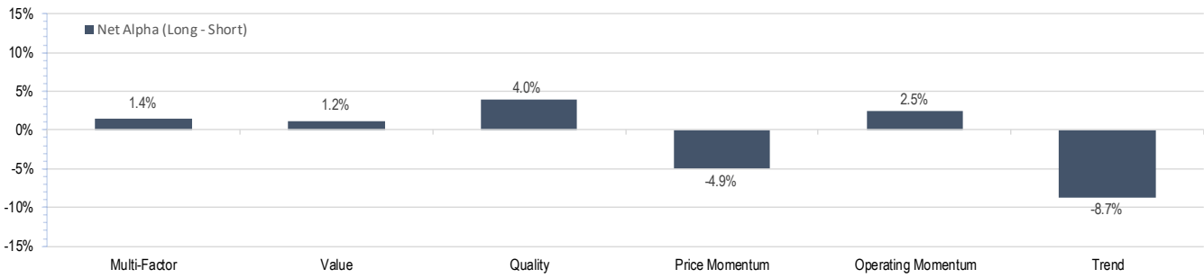
Multi-Factor Performance
