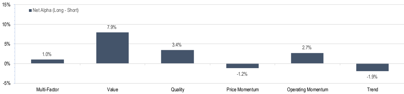
Multi-Factor Performance
