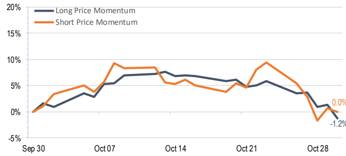
Trend Performance
